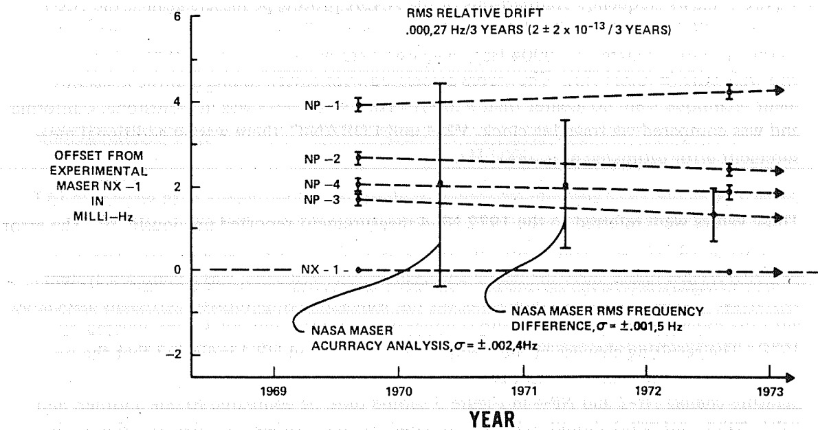
Figure 5. Frequency relationships—NASA NX-1 and NP-1, -2, -3, -4 atomic hydrogen masers.
