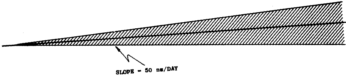
Figure 15. MAXIMUM TIME ACCUMULATION DUE TO SMALLEST INCREMENT OF IPS
