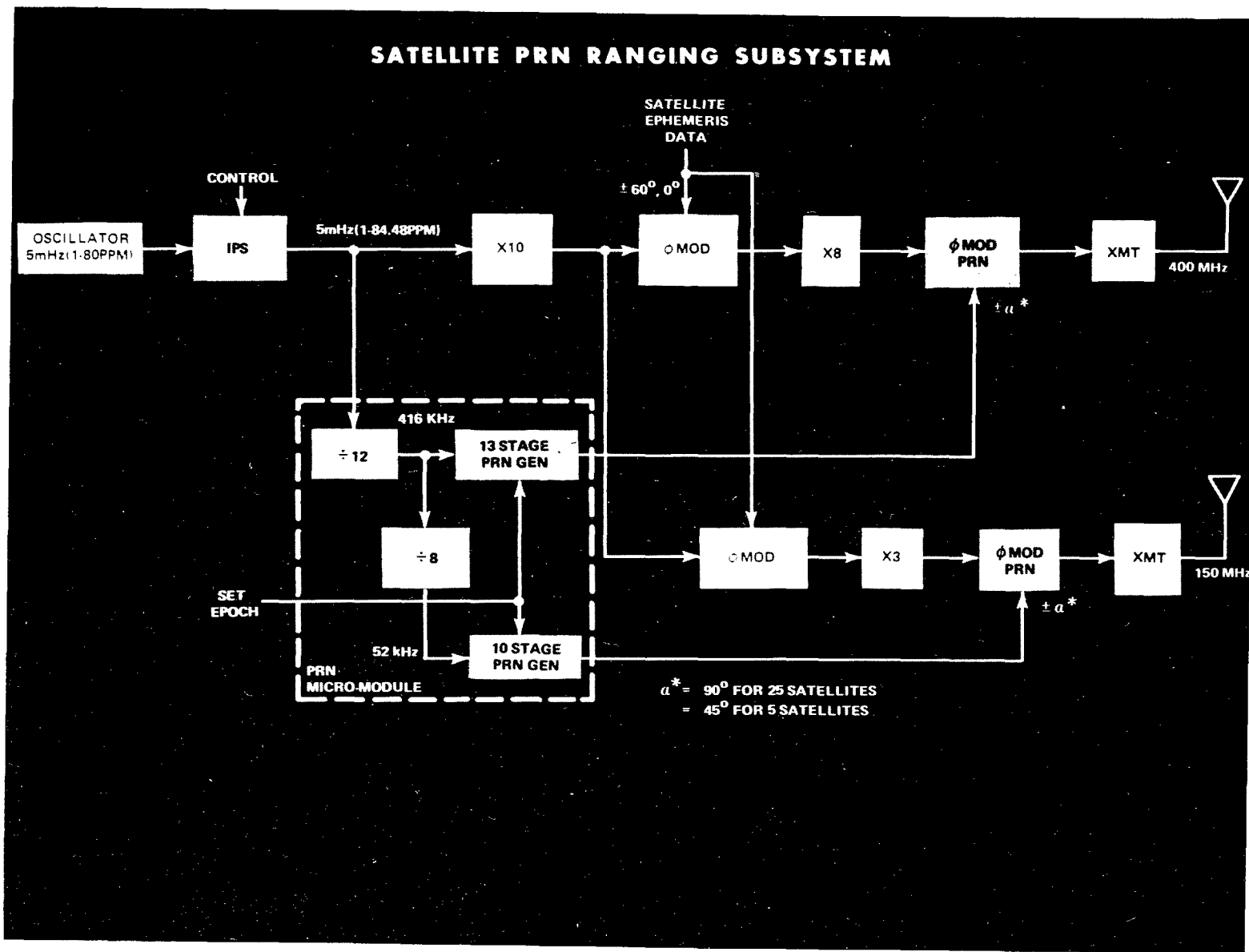
Figure 1. SATELLITE PRN RANGING SUBSYSTEM
