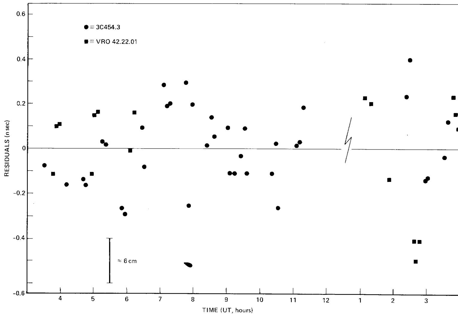
Figure 1. Postfit residuals from Observations of the Extragalactic Radio Sources VRO 42.22.01 and 3C454.3 during the Goldstone-Haystack VLBI Experiment of 29-30 August 1972
