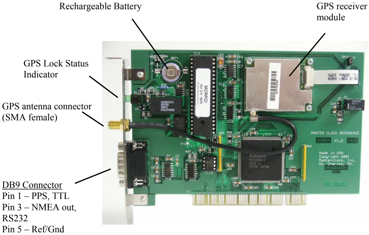
GPSPCI V1.2
