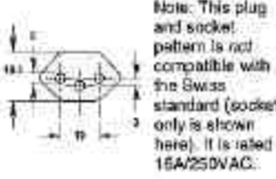
O IEC 908-1: "IEC System" for plugs & sockets
