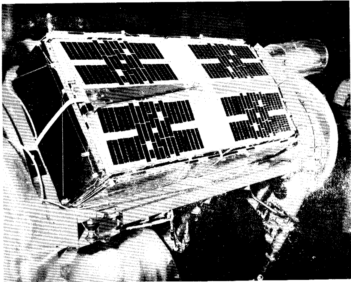
Figure 10. Timation II.
