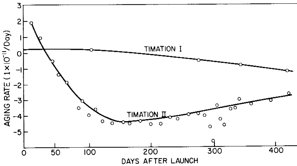
Figure 11. Aging rates of crystal oscillators.
