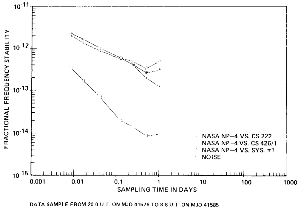
Figure 11. Frequency stabilities measurements – set I.
