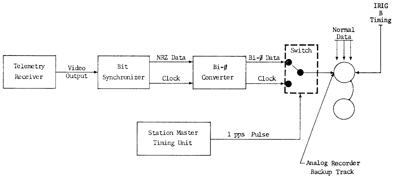
Figure 11. Real Time Telemetry Timing Marker System
