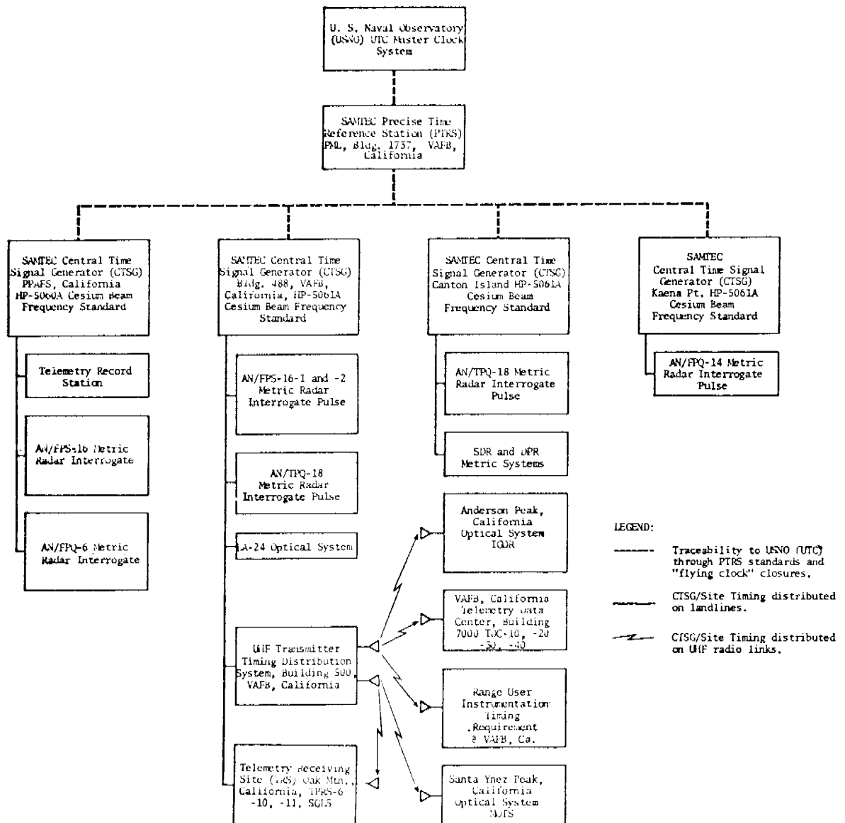
Figure 1. SAMTEC Instrumentation Systems UTC/IRIG Timing and Frequency Accuracy Traceability to USNO
