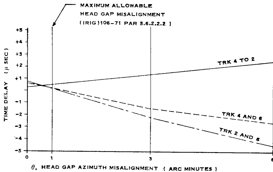
Figure 8. Time Delay Contributions Due to Recorder Head Gap Azimuth Misalignment
