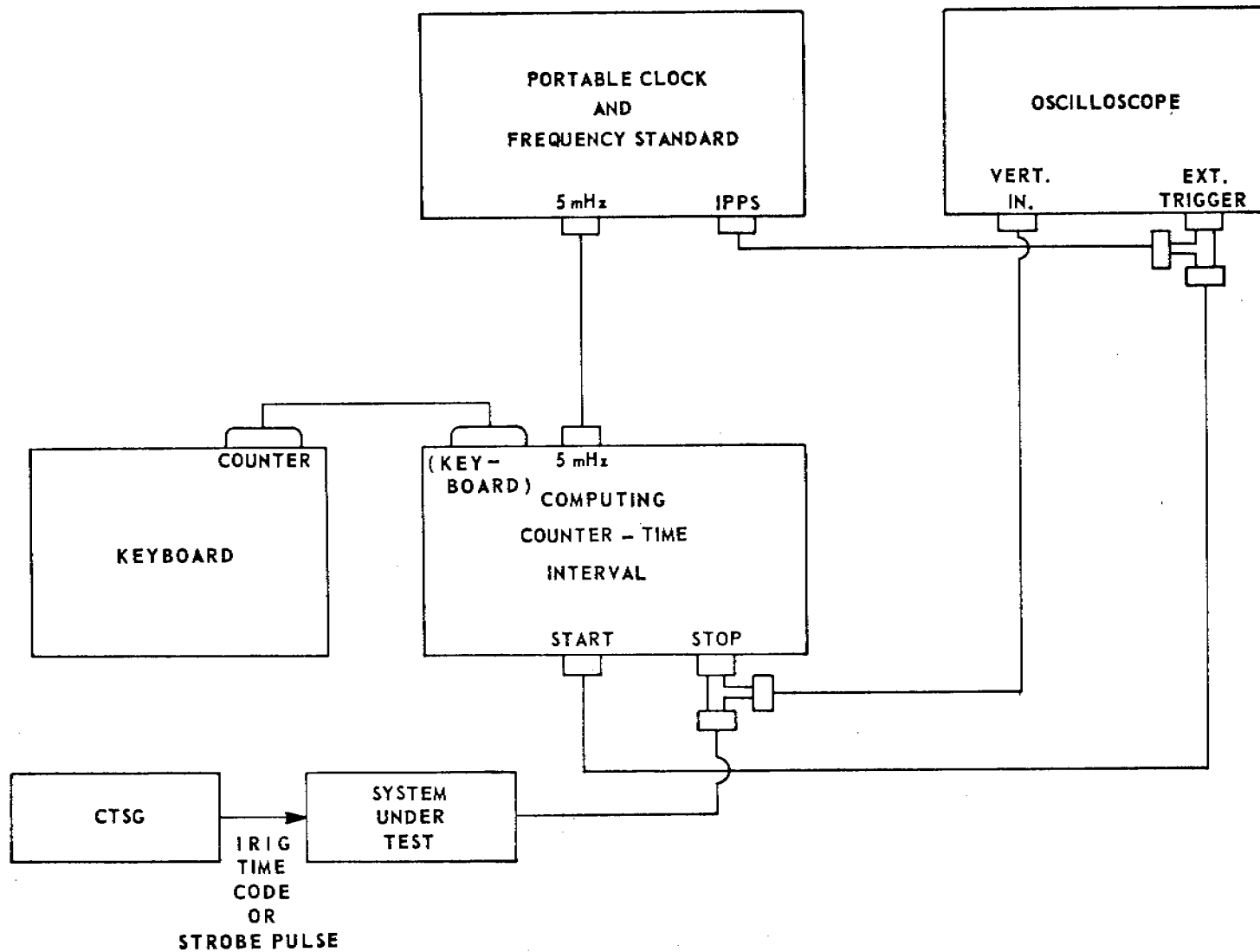
Figure 3. Typical Instrumentation Timing Accuracy Test Equipment Configuration
