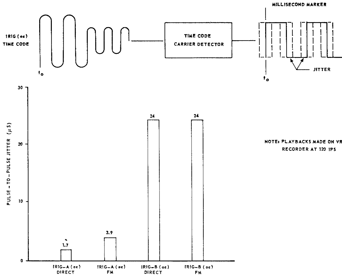
Figure 10. Examples of Pulse-to-Pulse Jitter Caused by the Time Code Translator
