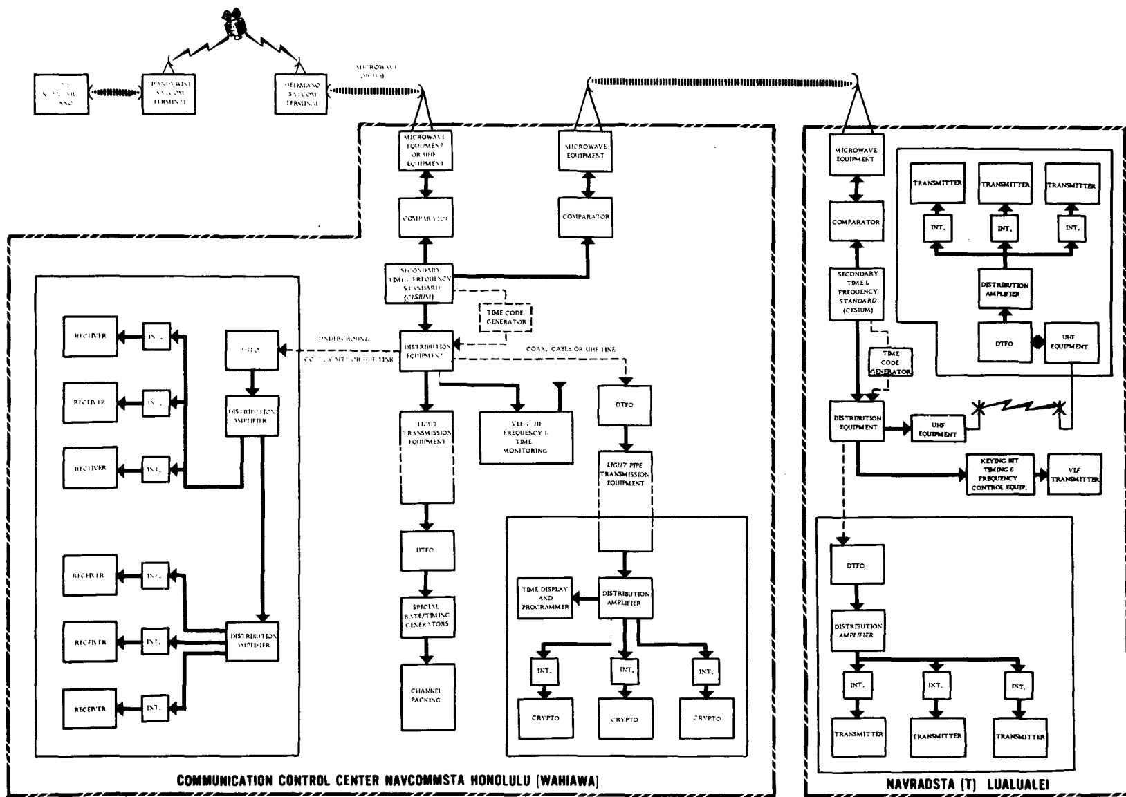
Figure 6. PRECISE TIME AND FREQUENCY LOCAL DISTRIBUTION FOR NAVCOMMSTA
